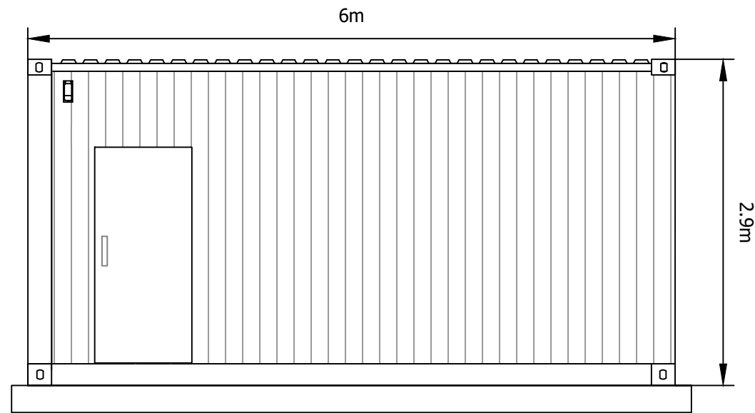
REAR ELEVATION
